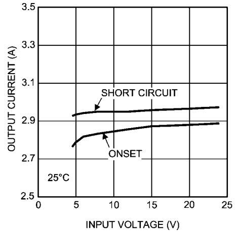
Current Limit 1.8V_{OUT} @ 25^\circ\text{C}
