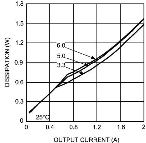
Dissipation 36V Input @ 25°C
