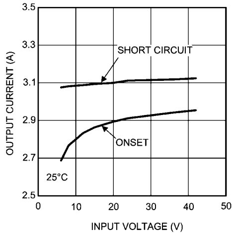
Current Limit 3.3V_{OUT} @ 25^\circ\text{C}
