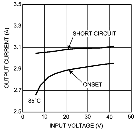
Current Limit 3.3V_{OUT} @ 85^\circ\text{C}
